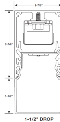
Luminaire Cross Section
